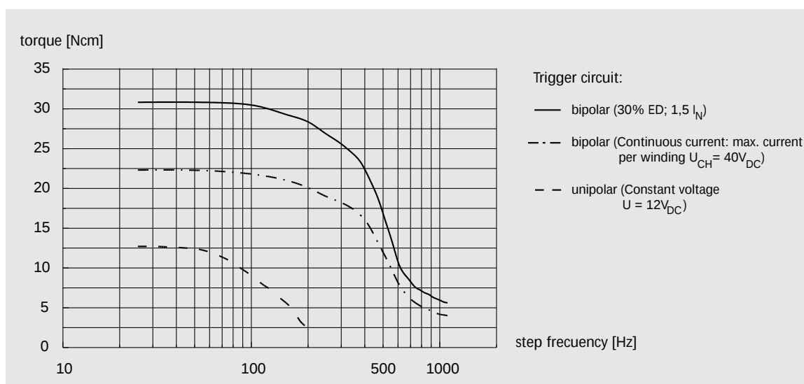
Characteristic curve RDM 63/10
