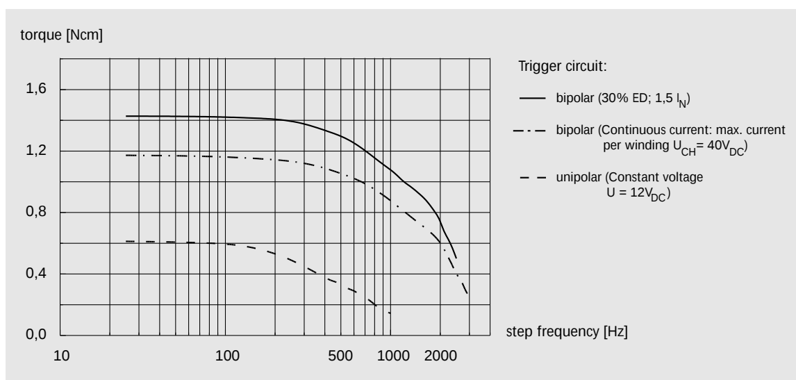
Characteristic curve RDM 36/12
