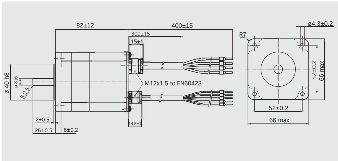
Scale drawing of the RECM 372/4
